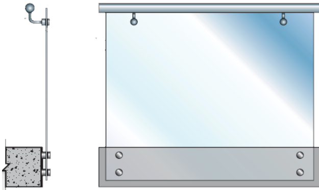
TG.3 - 12MM GLASS SIDE FIXED WITH RAIL FITTED OFF SIDE OF GLASS WITH BRACKETS
