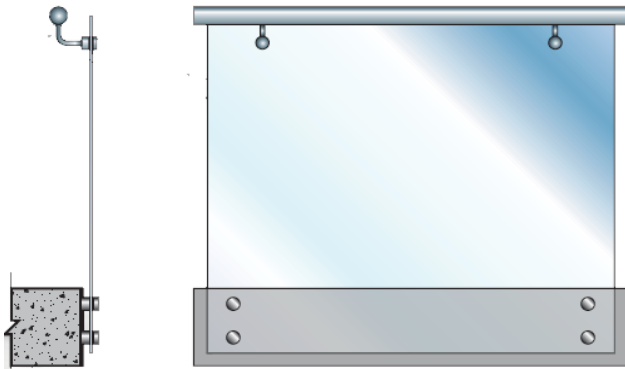
TG.3 - 12MM GLASS SIDE FIXED WITH RAIL FITTED OFF SIDE OF GLASS WITH BRACKETS
