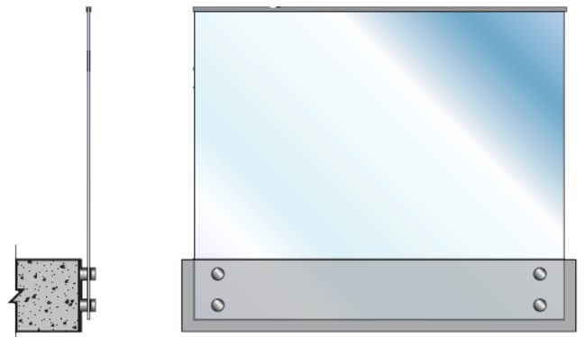
TG.4 - 12MM GLASS SIDE FIXED WITH RAIL FITTED TO TOP OF GLASS
