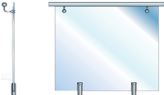
TG.5 - 12MM GLASS SPIGOT FIXED WITH RAIL FITTED OFF SIDE OF GLASS WITH BRACKETS
