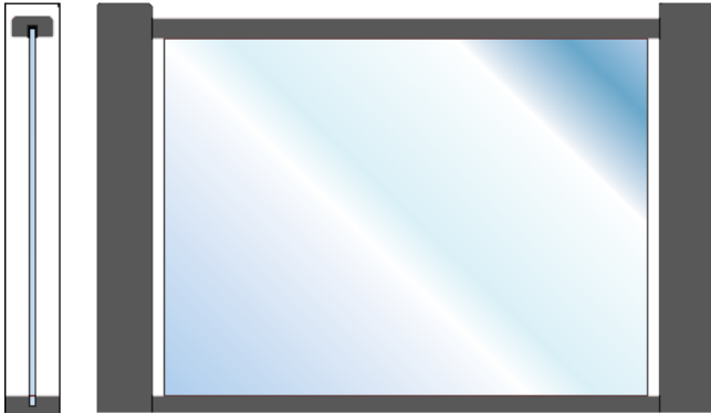
TG.1 - 10MM GLASS FITTED IN TIMBER RAIL & CAPPING BETWEEN TIMBER POSTS
