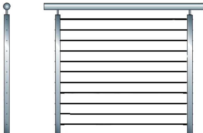
SSC.3 - S.STEEL CABLE BETWEEN S.STEEL 40X40MM SQUARE POSTS & RAIL FITTED TO POSTS
